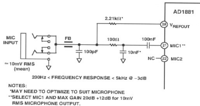
Figure 10. Microphone Input
